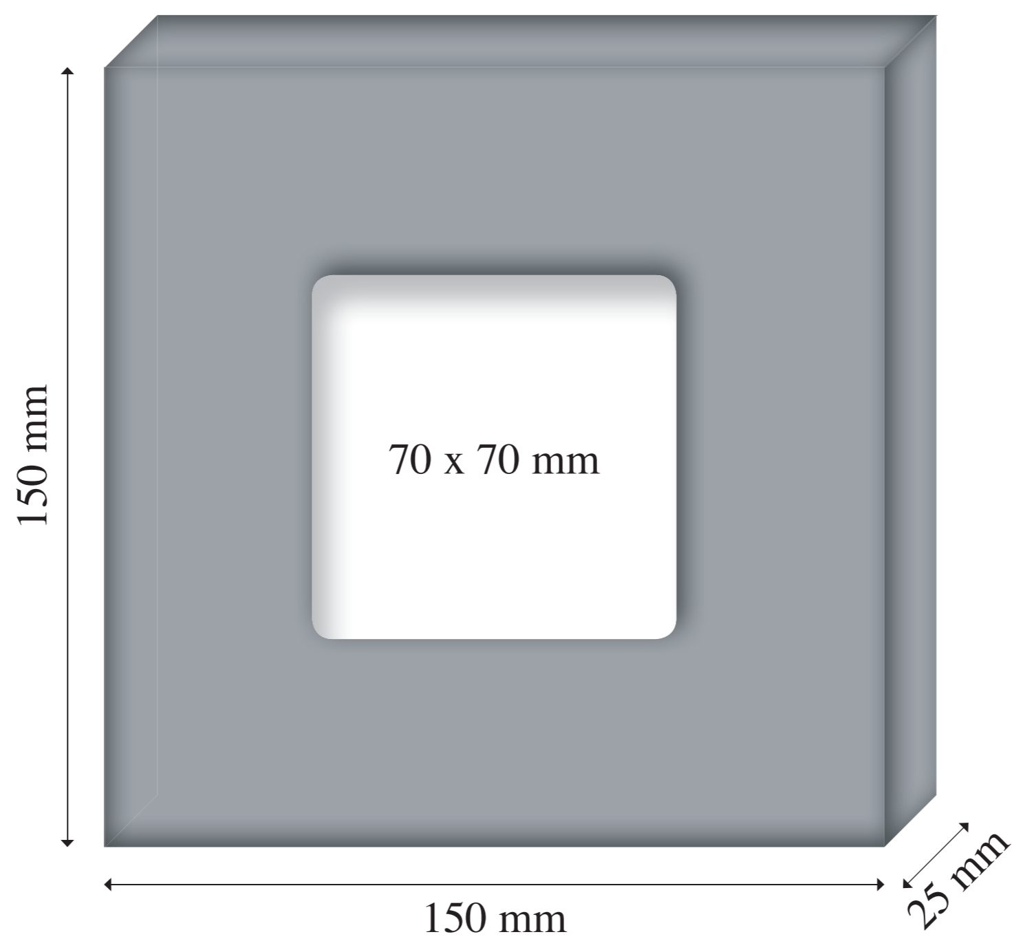
SILVER BOX 150 x 150 x 25 mm (Window: 70 x 70 mm)
